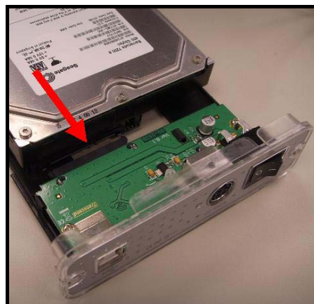
Figure 5. Connect the SATA hard drive to the SATA adapter
